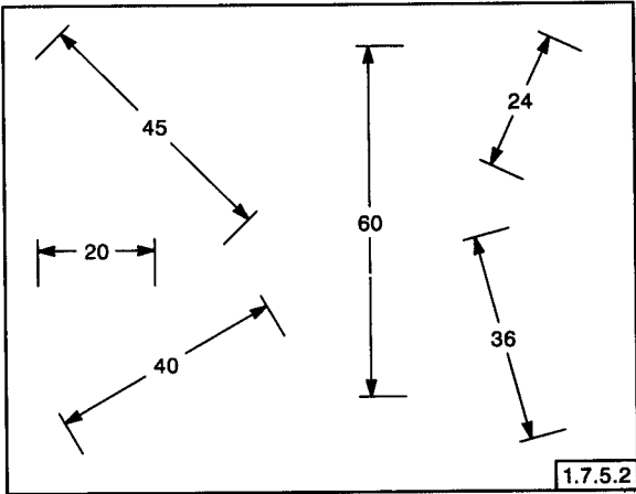
FIG. 1-16 READING DIRECTION
