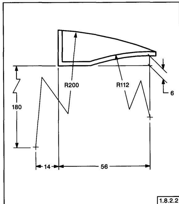
FIG. 1-23 FORESHORTENED RADII
