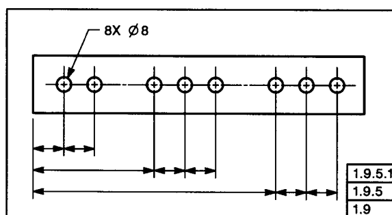
FIG. 1-52 REPETITIVE FEATURES
