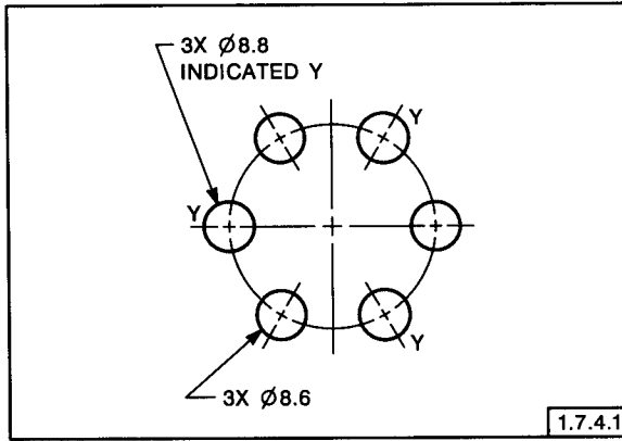
FIG. 1-14 MINIMIZING LEADERS
