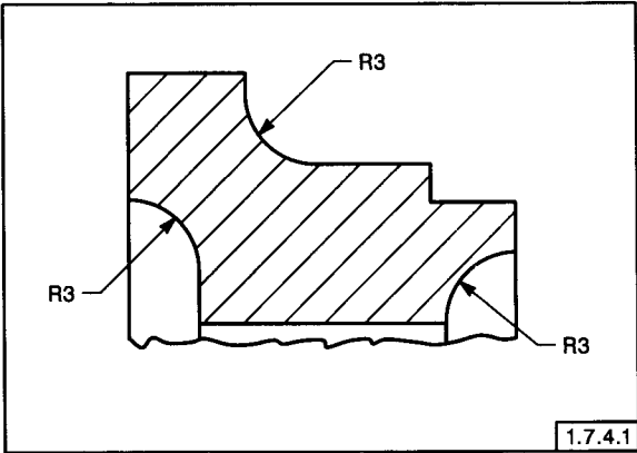
FIG. 1-13 LEADER-DIRECTED DIMENSIONS
