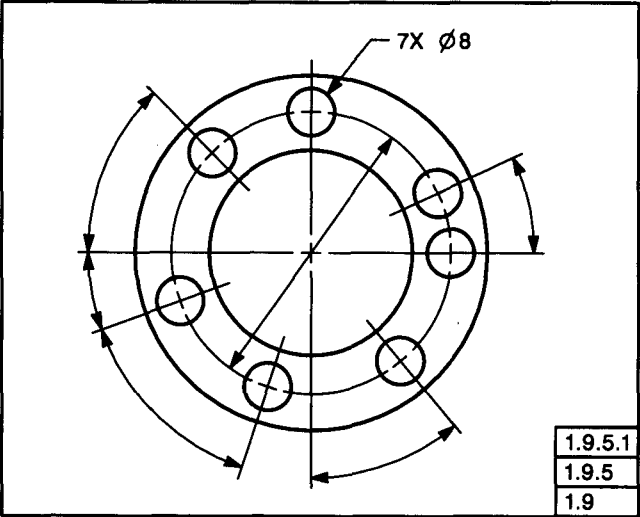
FIG. 1-53 REPETITIVE FEATURES
