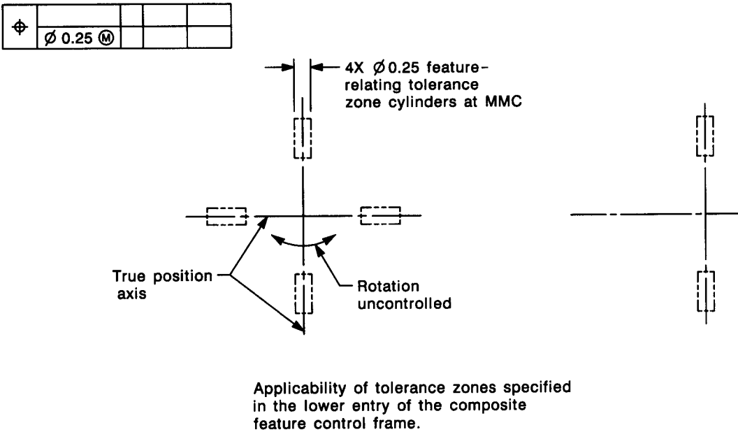
FIG. 5-25 RADIAL HOLE PATTERN LOCATED BY COMPOSITE POSITIONAL TOLERANCING (CONT'D) Tolerance Zones for Radial Hole Pattern
