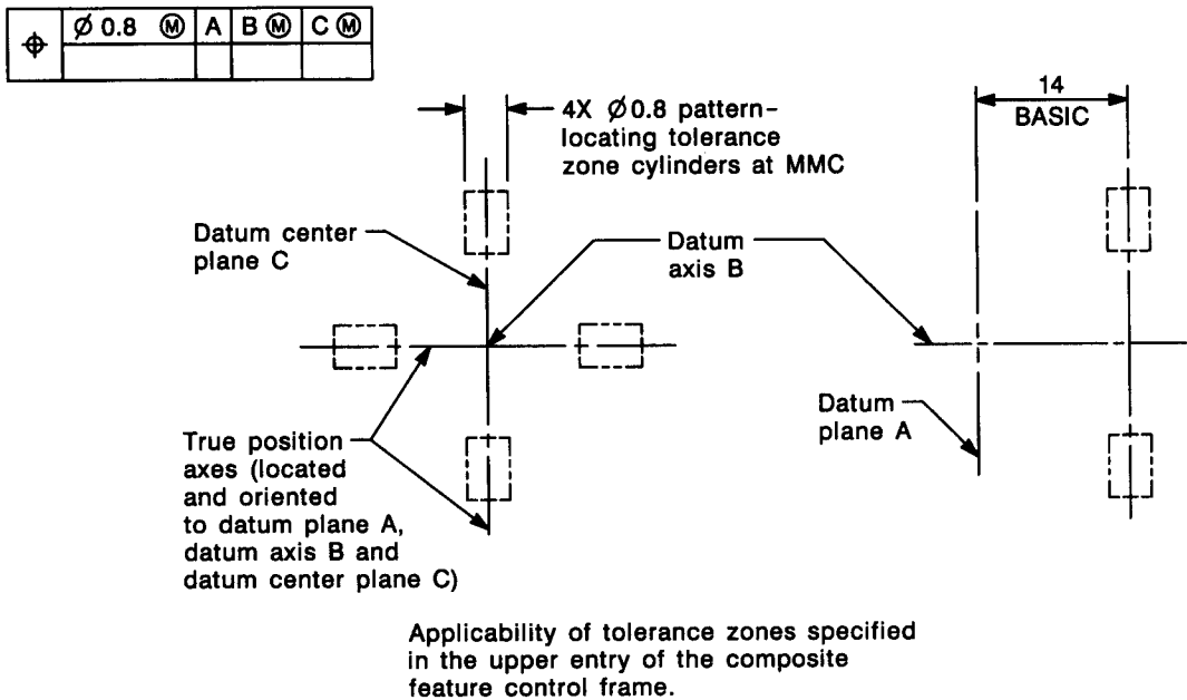
FIG. 5-25(b) FEATURE-RELATING TOLERANCE ZONE FRAMEWORK
