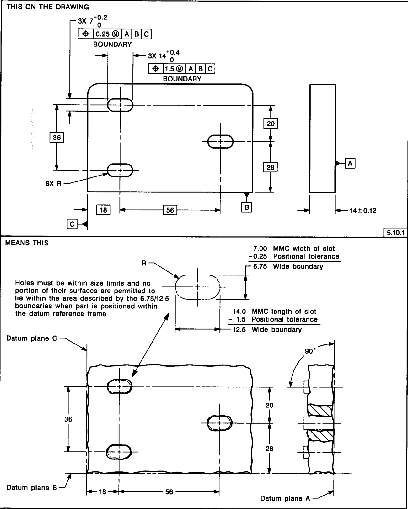
FIG. 5-47 POSITIONAL TOLERANCING OF ENLONGATED HOLES, BOUNDARY CONCEPT
