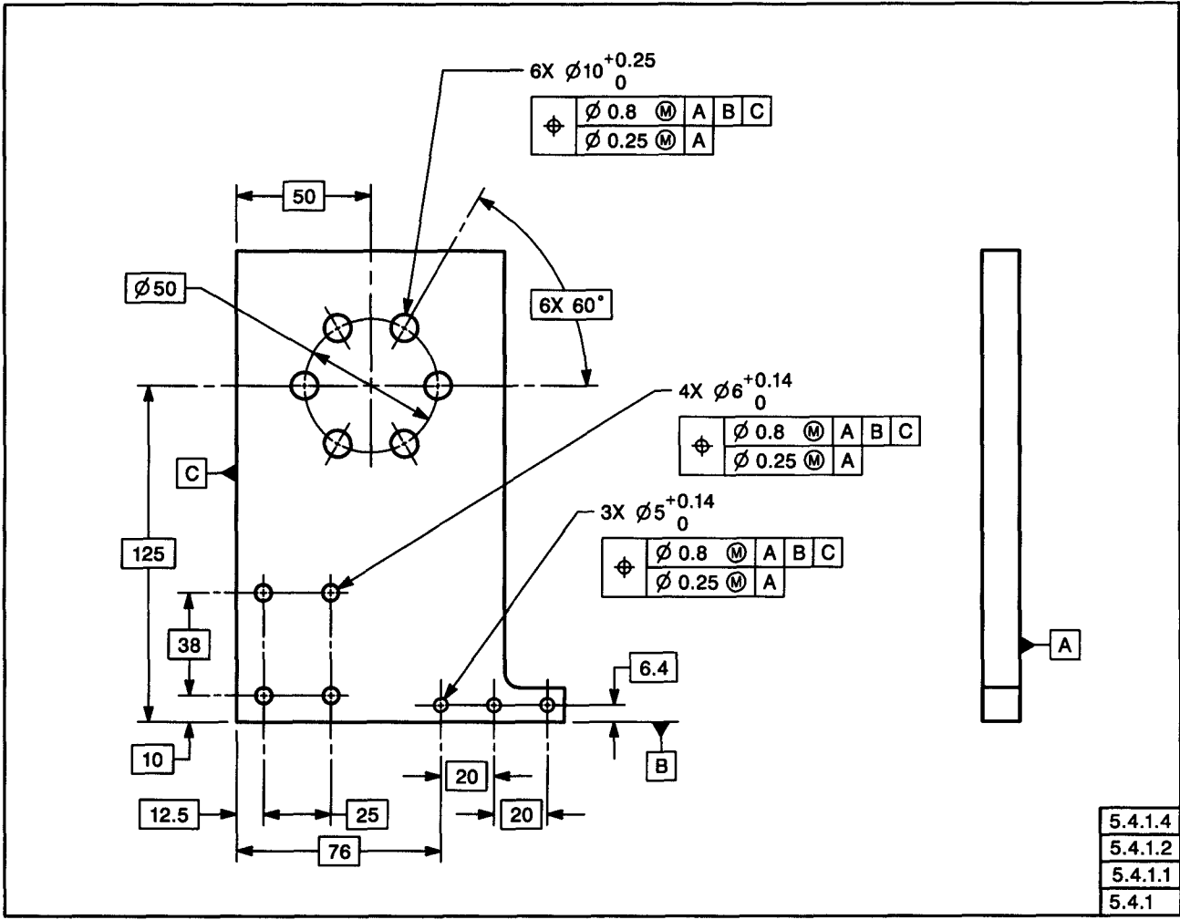
FIG. 5-19 HOLE PATTERNS LOCATED BY COMPOSITE POSITIONAL TOLERANCING
