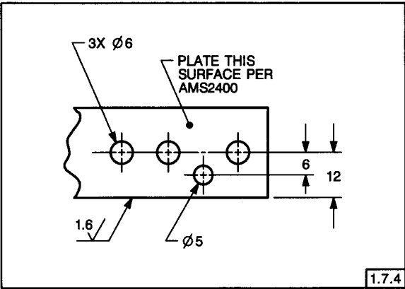
FIG. 1-12 LEADERS
